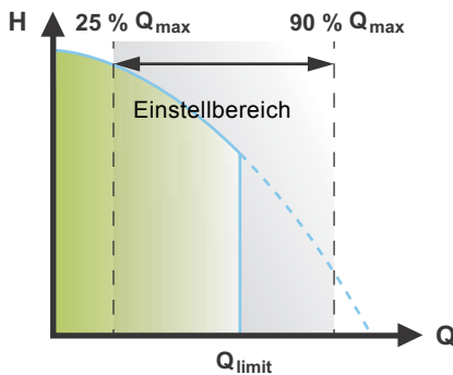
Abb. 45 FLOW LIMIT
