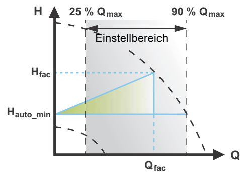
Abb. 35 FLOW_{ADAPT}
